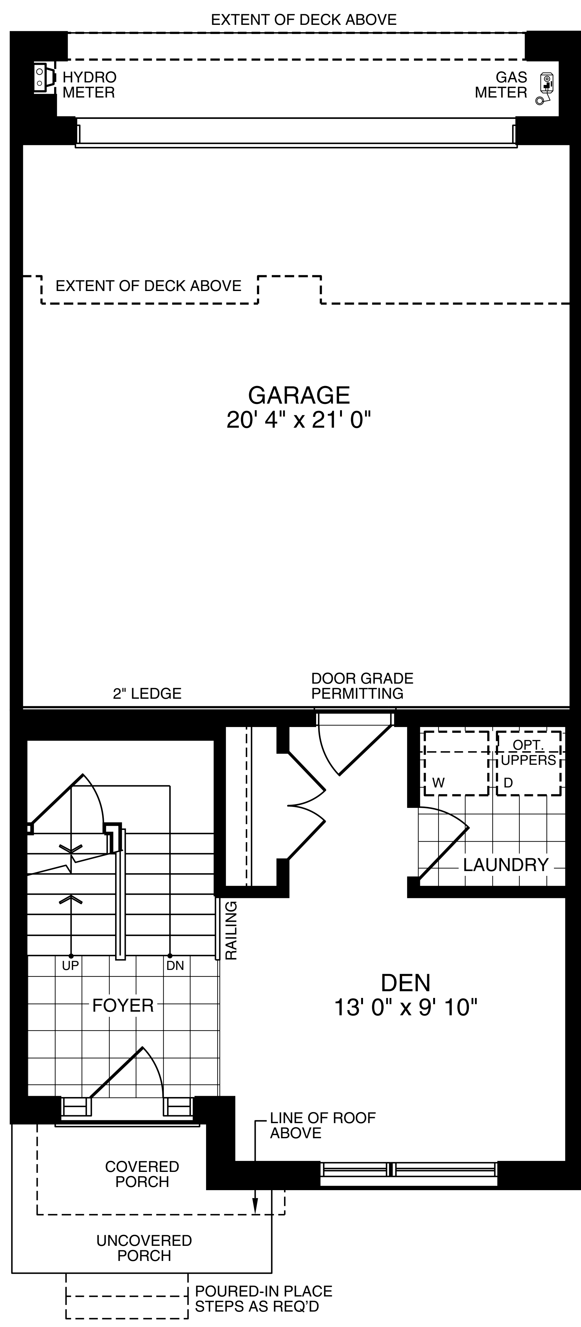
GROUND FLOOR PLAN ELEVATION A
